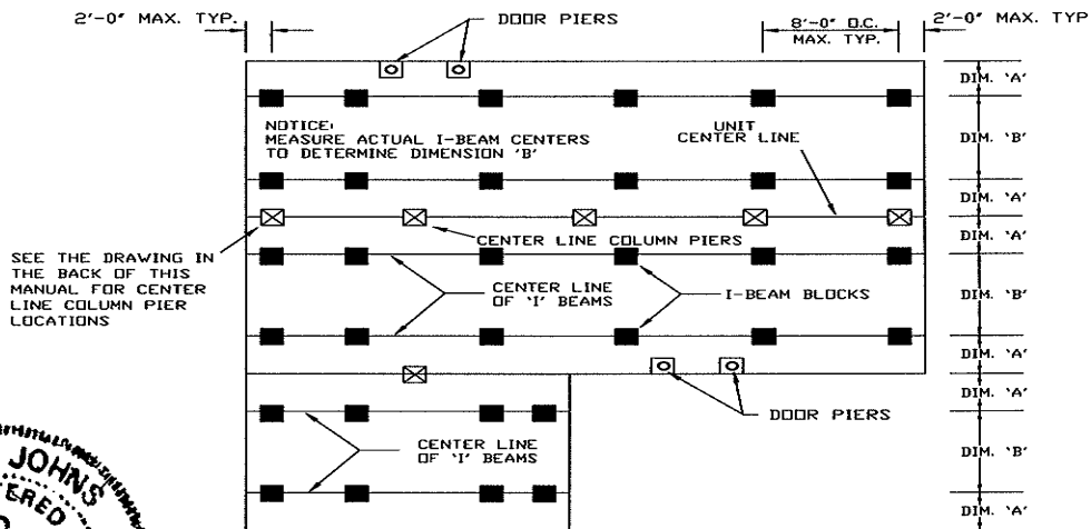
TYPICAL PERIMETER & FRAME SUPPORT FIGURE 4-4
