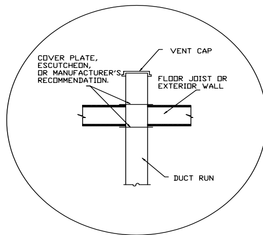
TYPICAL DRYER VENT
