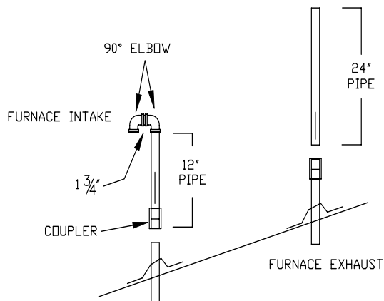
TYPICAL HIGH EFFICIENCY FURNACE STACKS (INTAKE & EXHAUST)
