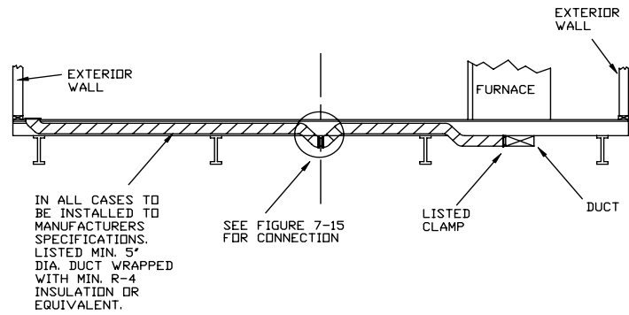
TYPICAL CROSSOVER CONNECTION
