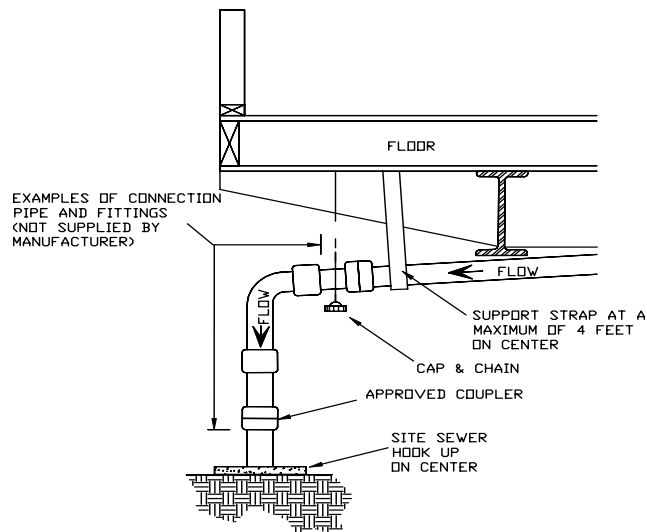
TYPICAL DRAIN CONNECTION
