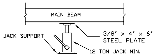
TYPICAL JACK PLACEMENT FIGURE 5-5
