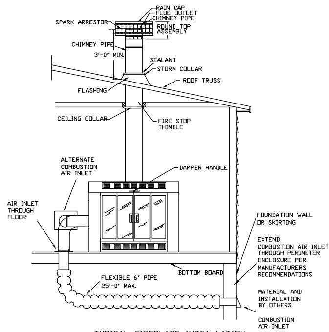
TYPICAL FIREPLACE INSTALLATION
