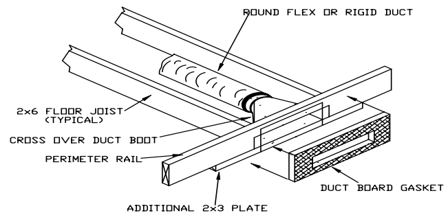
TYPICAL PERIMETER CROSSOVER
