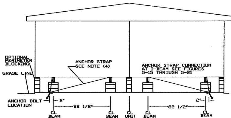
MAXIMUM ANCHOR SPACING (VERTICAL) 82 1/2" I-BEAM CENTERS ROOF SLOPE 7/12 ONLY
