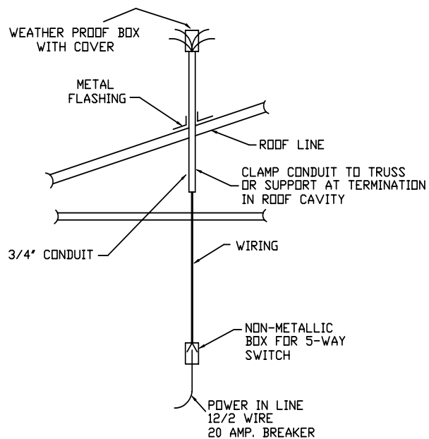
TYPICAL EVAPORATOR COOLER CONNECTION
