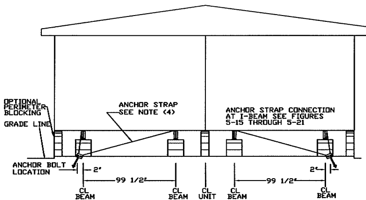
MAXIMUM ANCHOR SPACING (VERTICAL) 99 1/2" I-BEAM CENTERS ROOF SLOPE 5/12 ONLY
