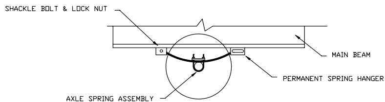
TYPICAL REMOVABLE AXLES
