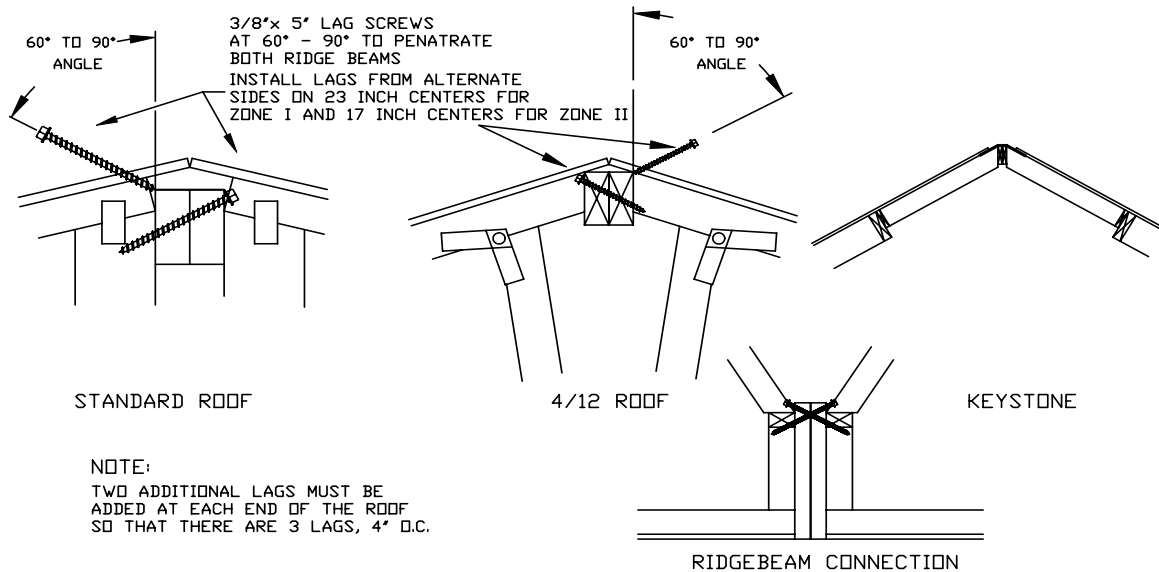
TYPICAL MARRIAGE LINE CONNECTION (RIDGEBEAM & ROOF)
