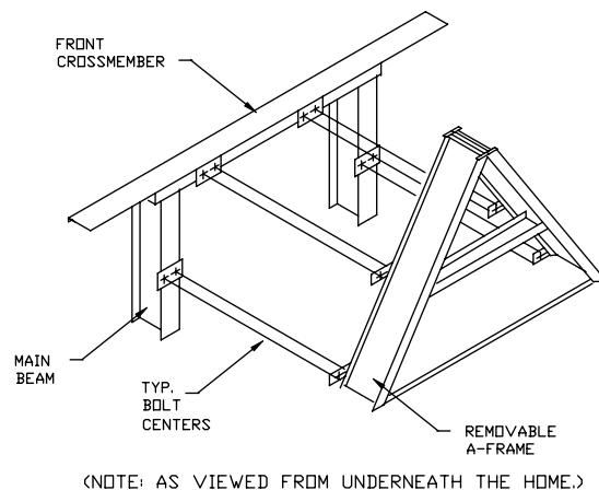
TYPICAL REMOVABLE A-FRAME
