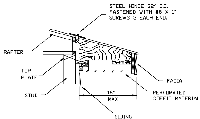
TYP. 16" HINGED EAVE. WIND ZONE 1
