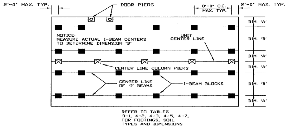
TYPICAL FRAME SUPPORT FIGURE 4-3
