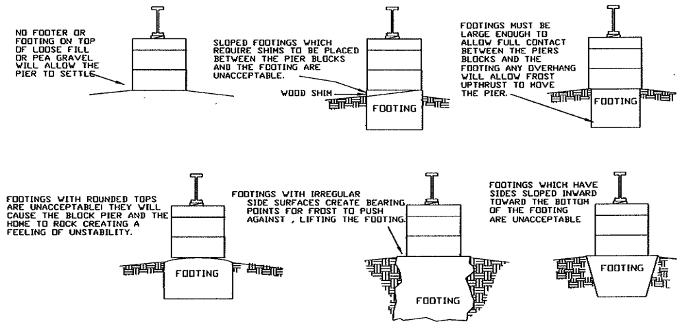
IMPROPER FOOTING DETAILS
