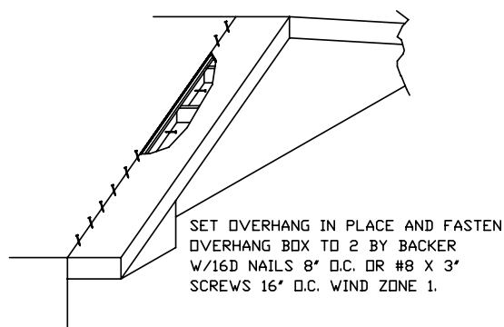
TYPICAL SHIPLOOSE OVERHANG
