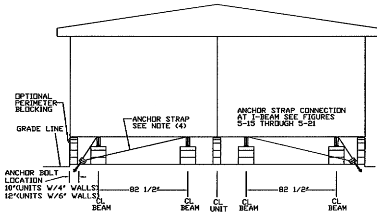
MAXIMUM ANCHOR SPACING (DIAGONAL) 82 1/2" I-BEAM CENTERS ROOF SLOPE 7/12 ONLY
