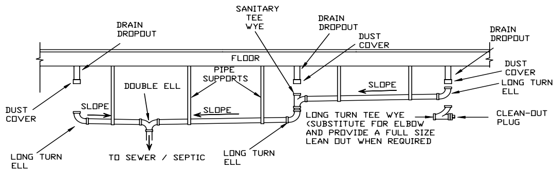
TYPICAL DRAIN CONNECTION
