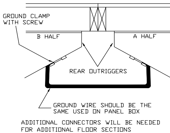
TYPICAL FRAME TO FRAME BONDING
