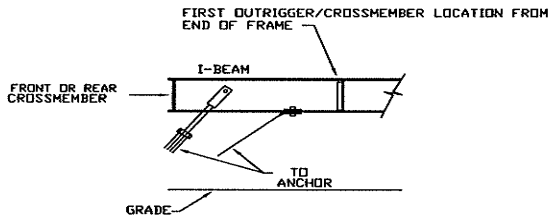
TYPICAL WIND ZONE II ANCHOR FASTENING FIGURE 9-22
