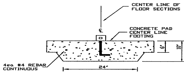
TYPICAL TIEDOWN FOOTER
