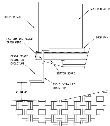
TYPICAL WATER HEATER DRAIN
