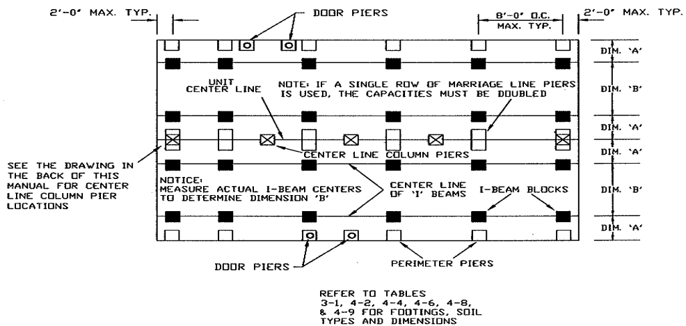
TYPICAL PERIMETER & FRAME SUPPORT FIGURE 4-4
