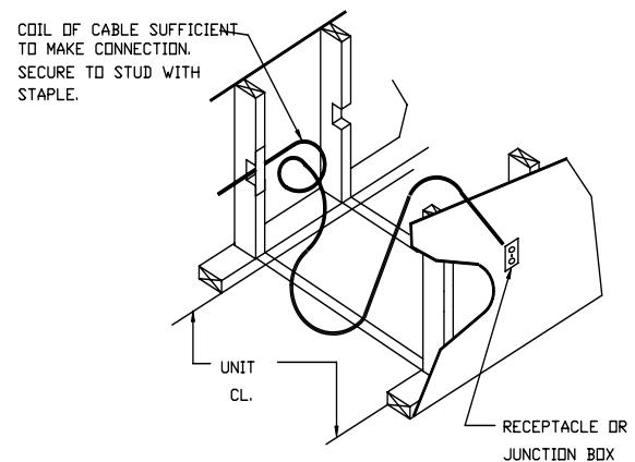
TYPICAL INTERIOR WALL CROSSOVER
