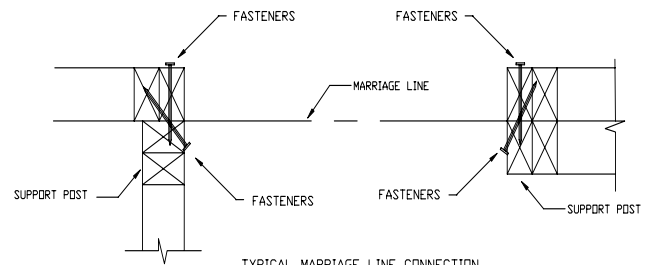
TYPICAL MARRIAGE LINE CONNECTION (COLUMN SUPPORTS) FIGURE 5-14
